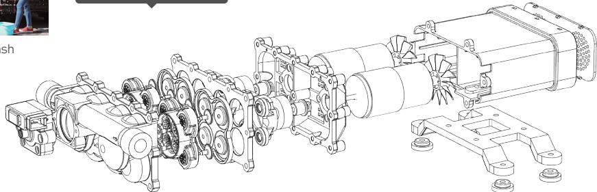
Dismantling Diagram
