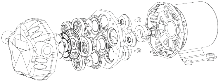
Dismantling Diagram
