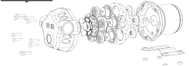
Dismantling Diagram
