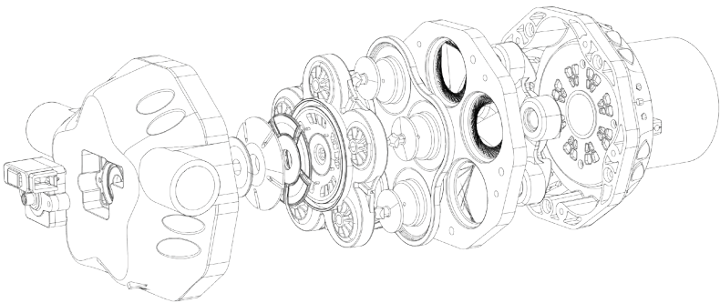
Dismantling Diagram
