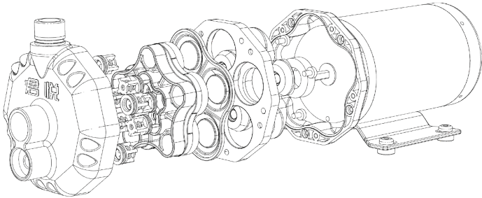
Dismantling Diagram
