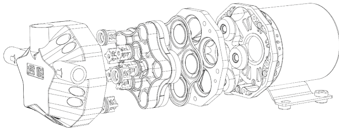
Dismantling Diagram
