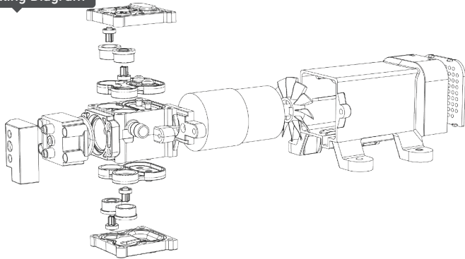
Dismantling Diagram
