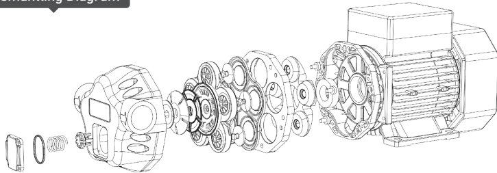
Dismantling Diagram
