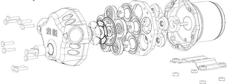
Dismantling Diagram
