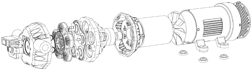
Dismantling Diagram
